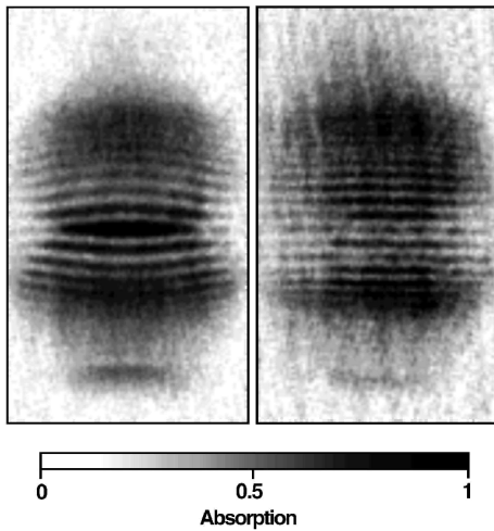
Figure 10.13: Interference patterns observed when two Bose-Einstein condensates overlap, arising from the constructive and destructive interference of the condensate wavefunctions with different phases.
