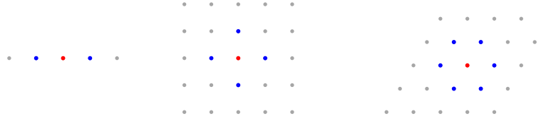
Figure 6.3: Comparison of coordination numbers z for lattices of increasing dimensionality: (a) one-dimensional chain ( z = 2 ), (b) two-dimensional square lattice ( z = 4 ), (c) two-dimensional triangular lattice ( z = 6 ), which has the same coordination number as a simple cubic lattice in 3D .
